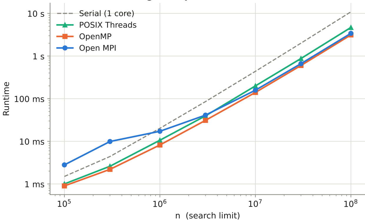
Runtime against problem size (4 workers)
